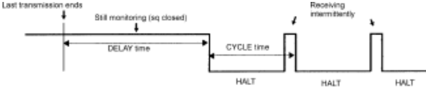
DELAY: Time between the last signal ended and the power save started CYCLE: The time between 'wake up' monitoring periods
